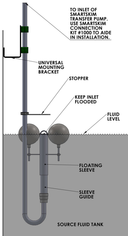
Typical 7" Skimmer Setup
